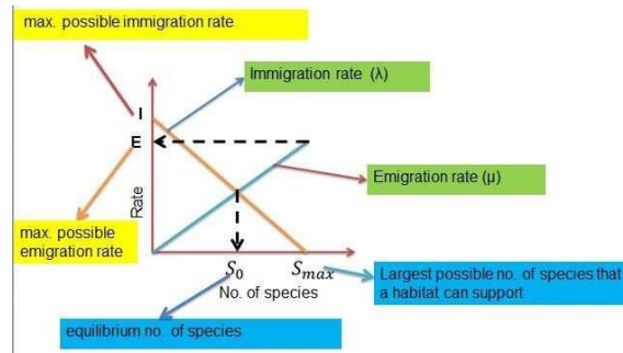
Fig. 1: Species Model [2]
